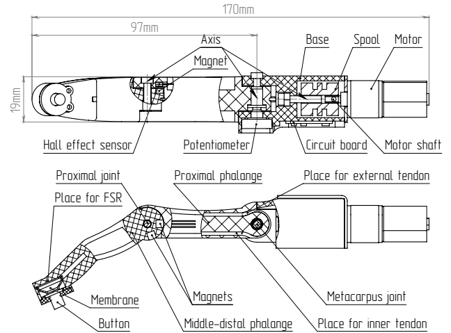
Fig. 2. Structure of 2-joint index finger
