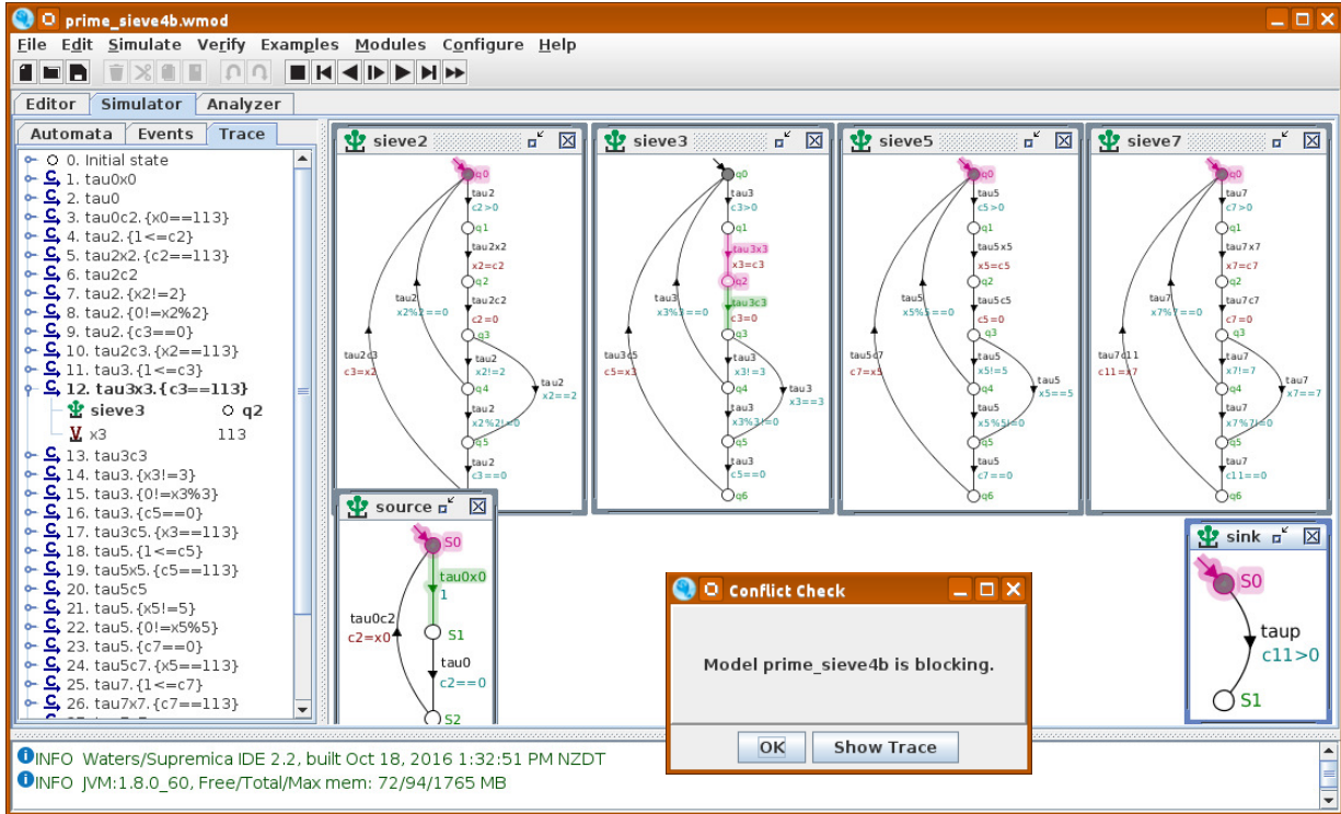
Fig. 1. Screenshot of counterexample simulation.
