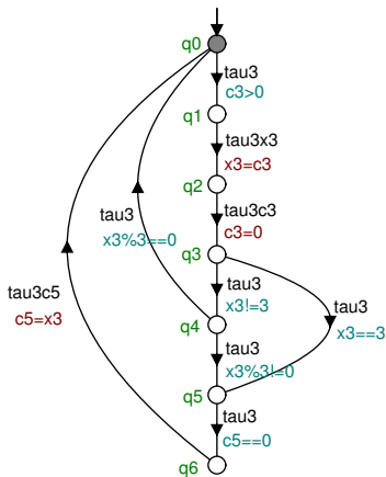
Fig. 2. Extended finite-state machine (EFSM).
